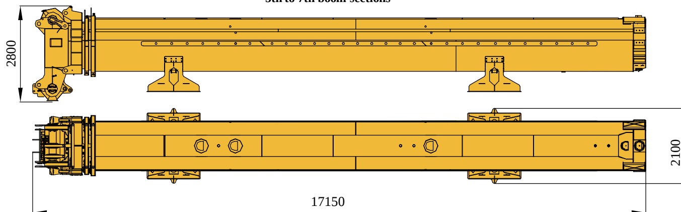
5-7节臂 27.8 t 5th to 7th boom sections
