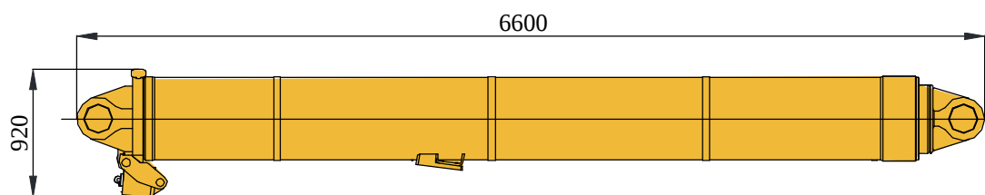
变幅缸 7 t Luffing cylinder
