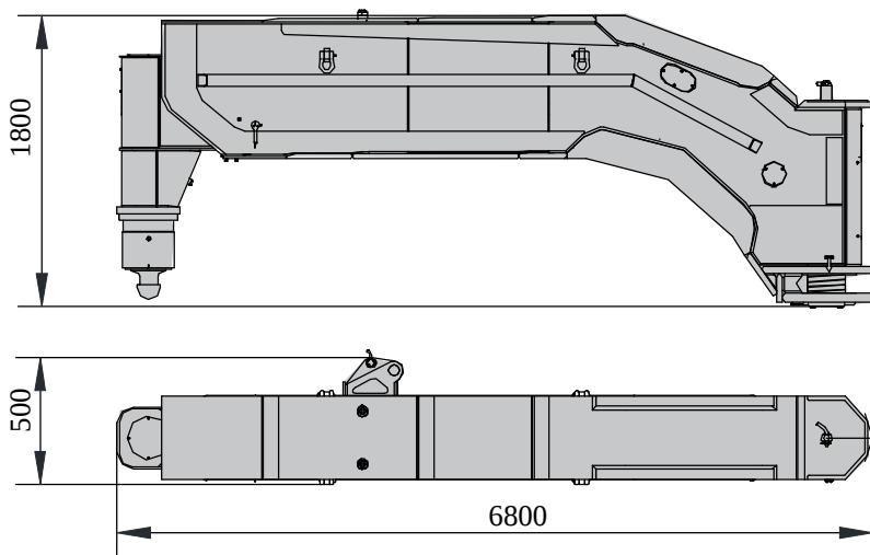
前支腿 7.8 t Front outrigger
