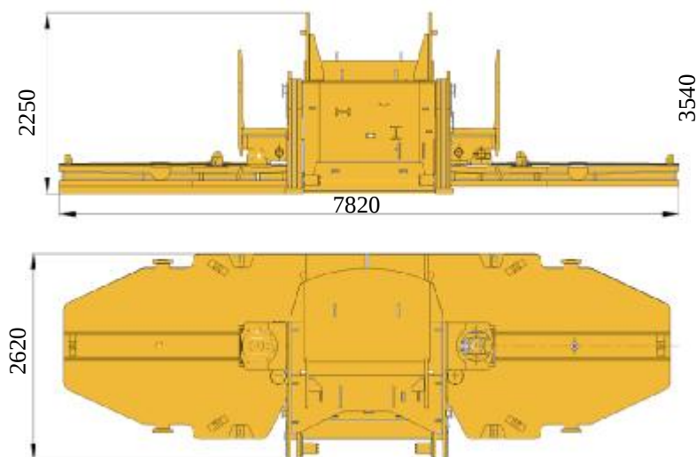
平衡重底座 35 t Counterweight base
