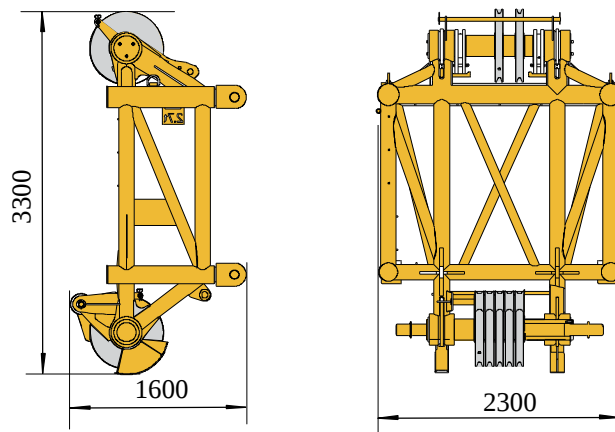
臂头 2.7 t Head section
