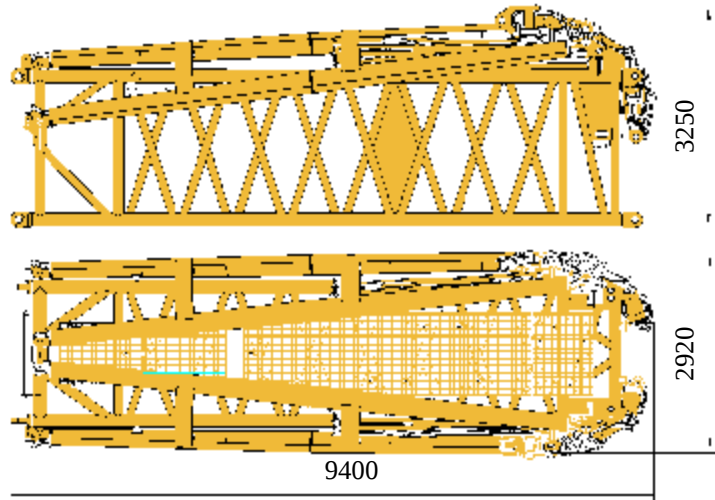
翼式连接架 11.6 t Wing-type connecting bracket
