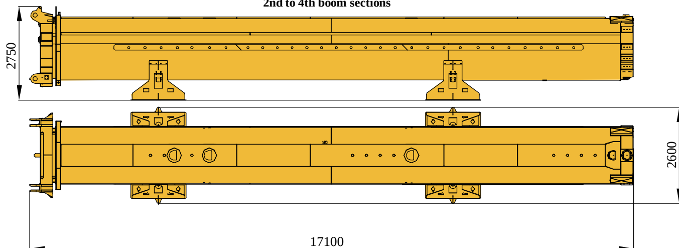
2、3、4节臂 31 t 2nd to 4th boom sections
