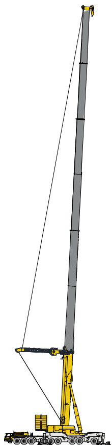
超起+主臂 Super lifting device+ boom
