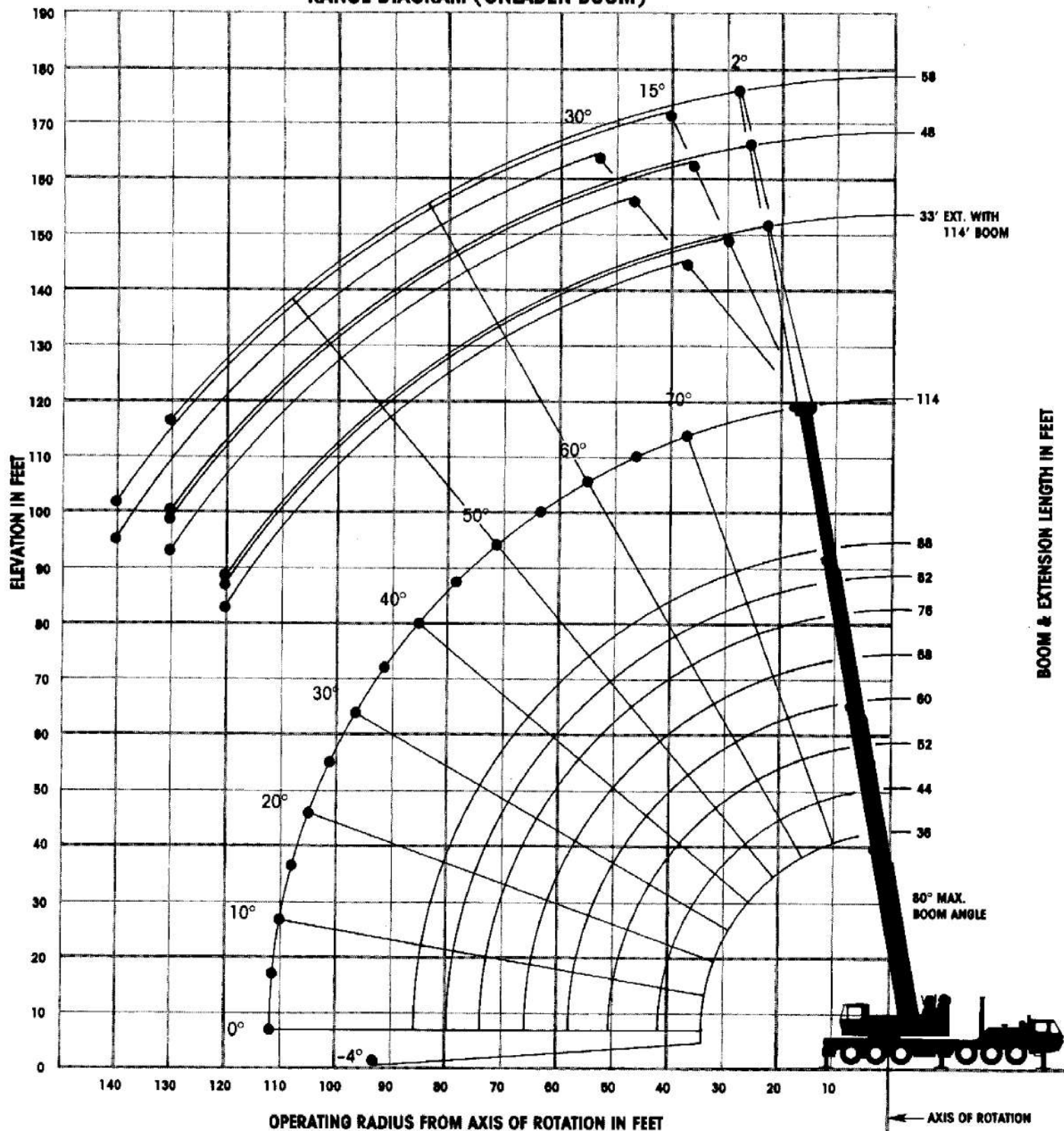
RANGE DIAGRAM (UNLADEN BOOM)
